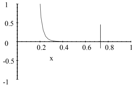
Figure 3. Distribution of the function of local warming K(x) when t = 1P \sim \Omega_0^{-1} . Disturbance of the inflow reaches \sim 731-732R_g .
