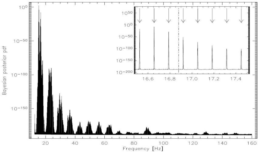
Figure 2. Application of the GL method for blind periodicity search to the complete data set obtained by RXTE PCA of giant flare of SGR 1806–20 2004 Dec 27 revealed a strong coherent signal at the frequency of 0.13219244 Hz and higher harmonics up to 100Hz. Bayesian posterior probability density vs frequencies in the range of 12.0–160 Hz is shown. The inset panel shows a zoomed part of it around 16.88 Hz. Arrows are indicating higher harmonics (from 125 to 132) of the fundamental frequency and the dash-dotted vertical line shows one of the detected QPO frequency in a short time interval (see text, for details).
