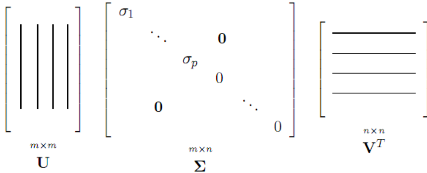
Figure 1. Structure of SVD matrices decomposition.
