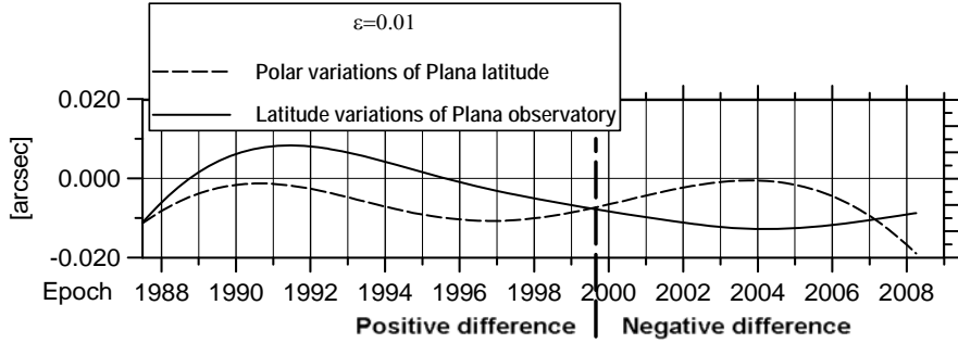
Figure 3. Vondrák-Whitaker filtration of the latitude variations of Plana observatory and polar variations of Plana latitude determined with smoothing factor \epsilon=0.01 . The nonpolar latitude changes are positive before 1999.6 and dominating negative after.
