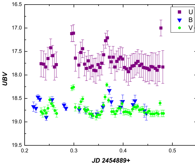
Figure 4. The simultaneous about 6 hours lasting observations of KR Aur on February 26, 2009 in UB.
