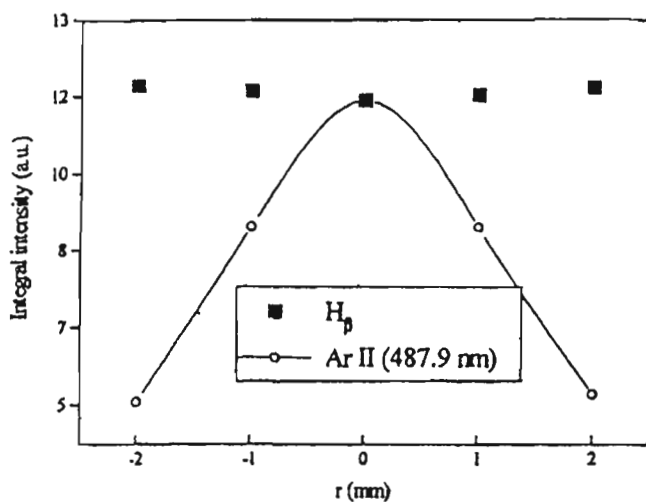
Fig 3. Radial distributions of the H β and Ar II (487.9 nm) spectral lines integral intensity. Discharge conditions: Direct polarity mode; p =100 Pa; I=25 mA; U = 255V.
