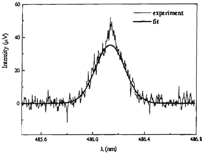
Fig. 2. The recording of H_{\beta} line profile at radial distance r=1 mm from optical axis of CMCD and its best fit. Discharge conditions: Direct polarity mode; p=100 Pa; I=25 mA; U=255 V.
