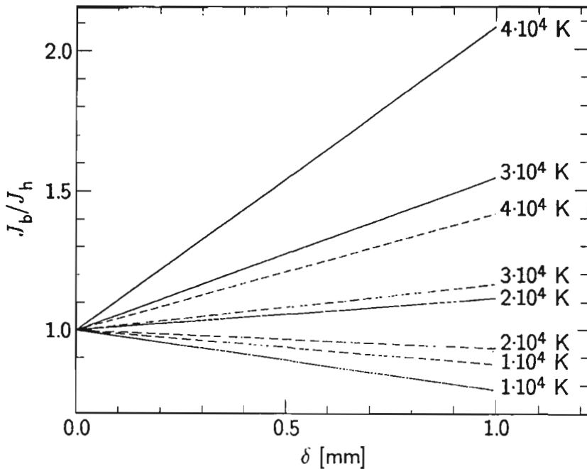
Fig. 1. Ratio of total line intensities influenced by boundary layers J_b / J_h / homogeneous plasma J_h , as function of the boundary layer thickness for electron concentration of N_e = 1 \cdot 10^{22} \text{ m}^{-3} (solid lines) and N_e = 5 \cdot 10^{23} \text{ m}^{-3} (dashed lines).
